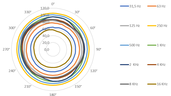
Directivity 1/1 OCT
