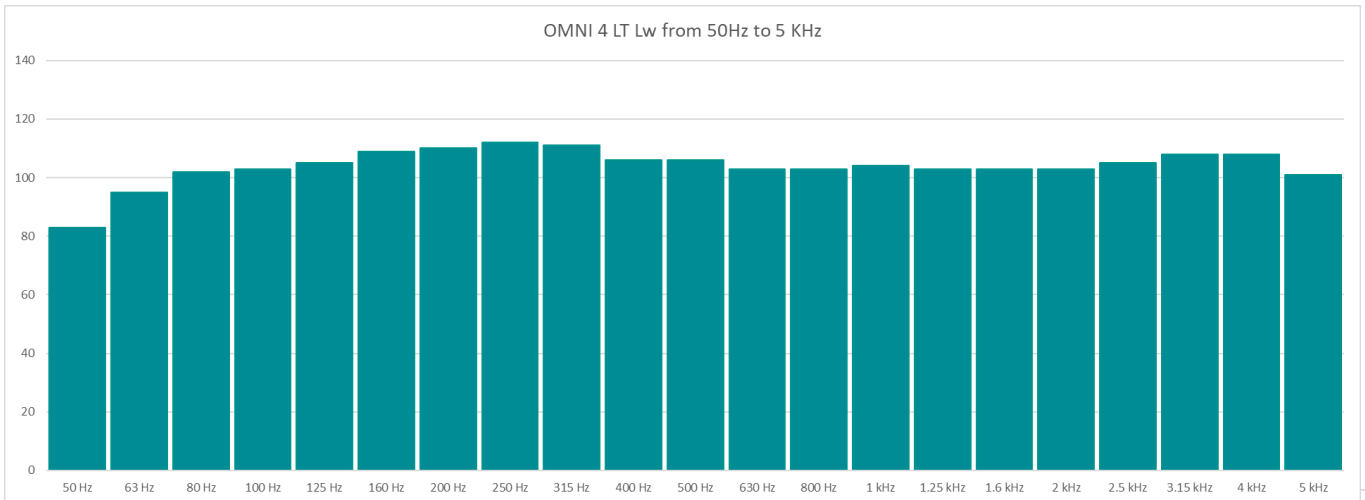
Sound Power Level (Lw) vs frequency of the Omni 4" LT
