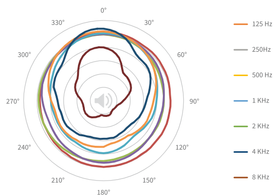
1/1 OCT DIRECTIVITY
