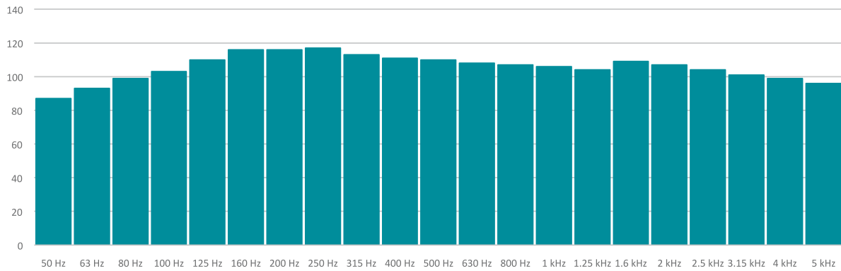
Sound Power Level (Lw)
